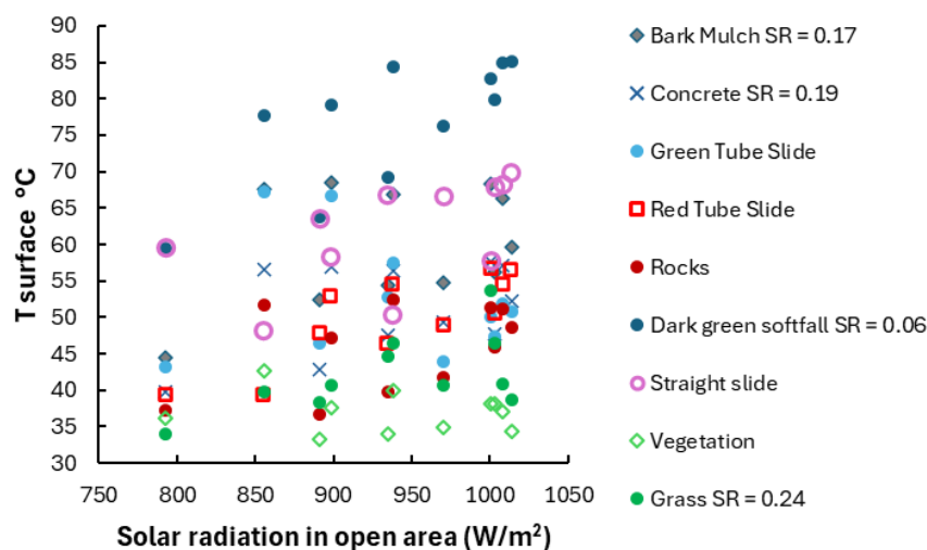
Figure 46. Surface temperature of the different materials as a function of incoming solar radiation measured at North Rocks Park Playground on 07/02/2025.
